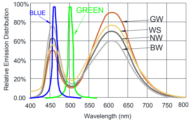
Wavelength Characteristics
